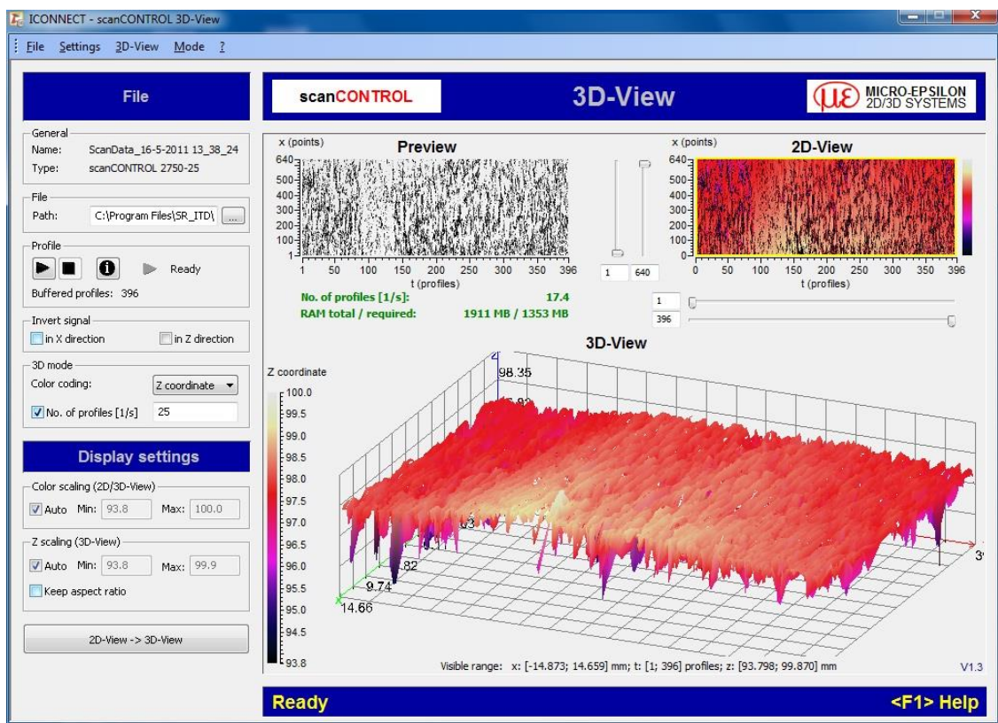
Figure 10: Typical output of surface roughness measurement
