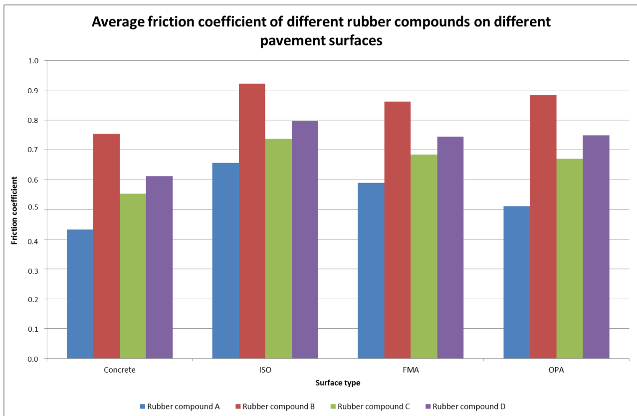
Figure 19: Test results of skid resistance of different rubber compounds on different surface layers.
