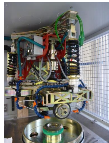
Figure 3: The SR-ITD set-up
